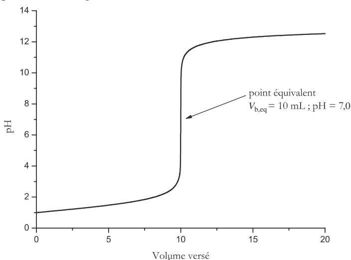
FIGURE 7.14 – Évolution \text{pH} = f(v)
